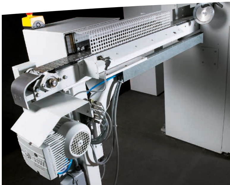
Cut piece outfeed conveyor with sliding device ("to the left" version)
